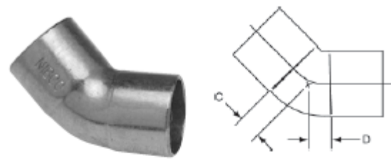
606 45° Elbow C x C – Wrot
